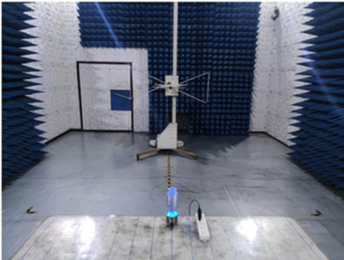
Radiated emissions at frequencies up to 1 GHz
